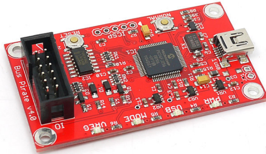
Figure 3.2: Bus Pirate v.4 (photo taken from [36])
