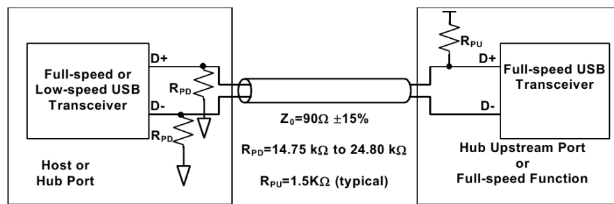
Figure 4.4: Pull-up and pull-down resistors of a Full Speed function, as prescribed by the USB specification rev. 2.0
