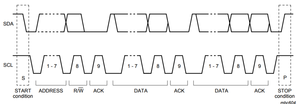
Figure 7.4: An I 2 C message diagram. (Diagram taken from the I 2 C specification UM10204 by NXP Semiconductors)
