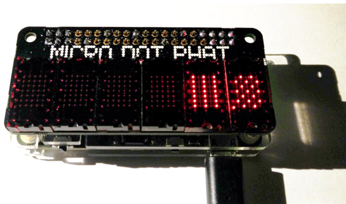
Figure 14.1: GEX Zero with the Micro Dot pHAT add-on board showing a test pattern
