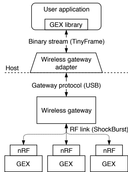
Figure 13.2: A block diagram of the wireless connection
