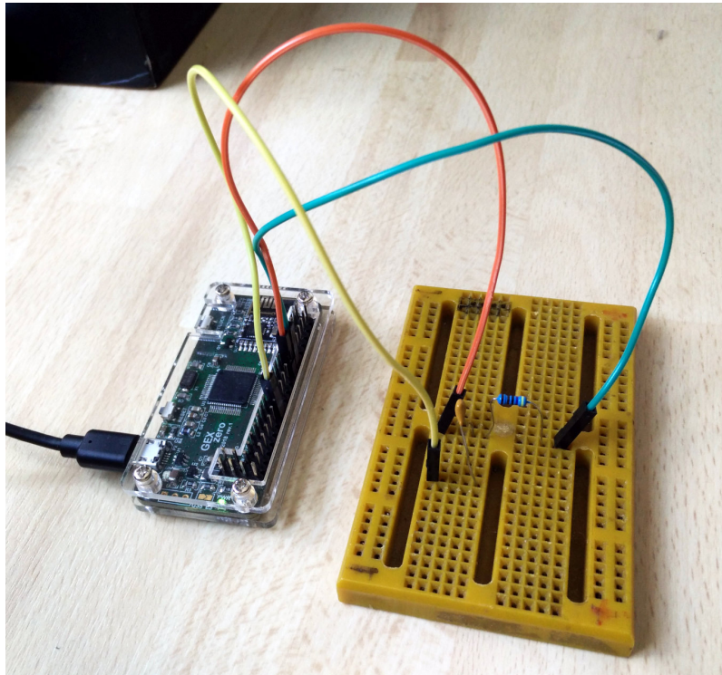
Figure 18.1: GEX Zero measuring a passive high-pass RC filter
