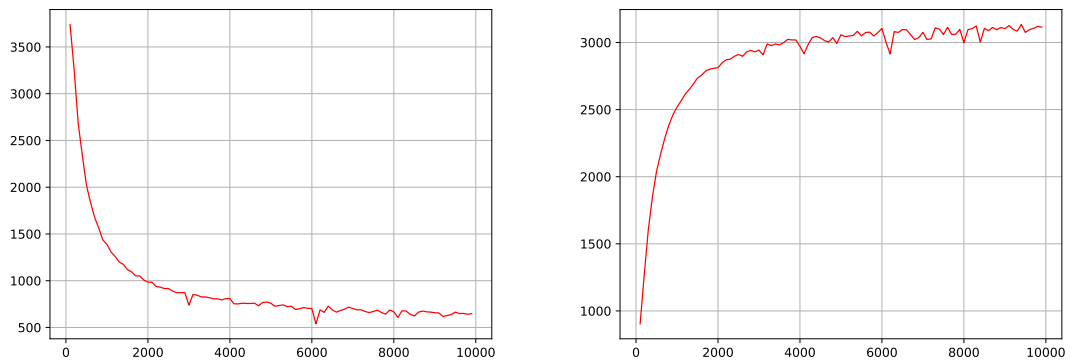
Figure 18.2: Frequency response of two complementary passive RC filters, captured by GEX controlled with a Python script. X: frequency (Hz), Y: peak-to-peak voltage as a raw ADC word
