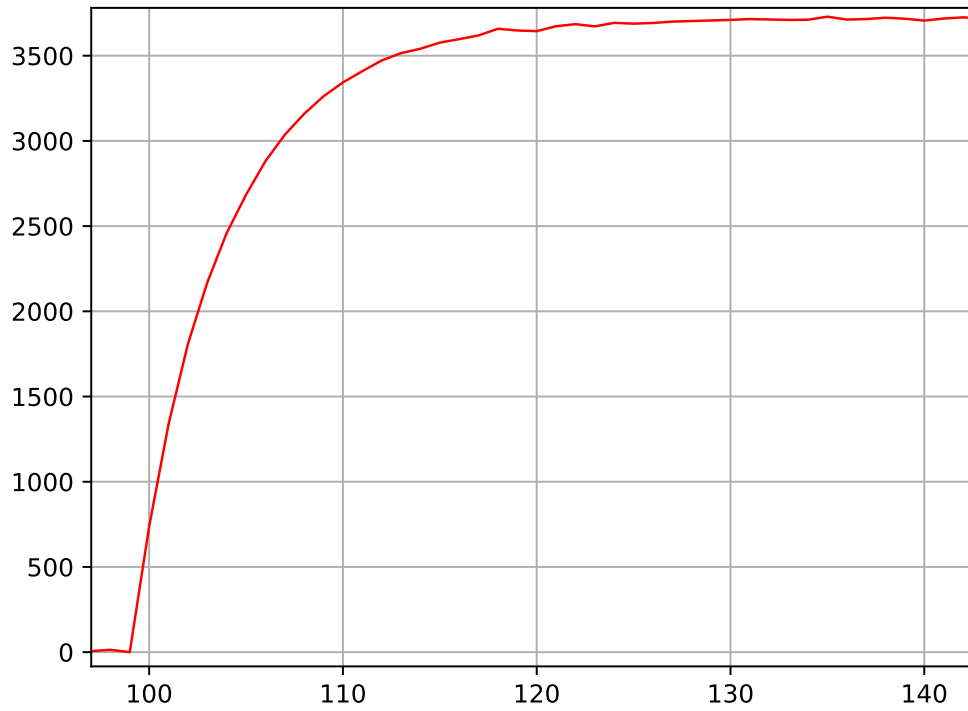
Figure 18.4: Capacitor charging waveform captured by the ADC unit, 50 kS/s. X: sample number, Y: ADC word. X grid: 200 \mu s.
