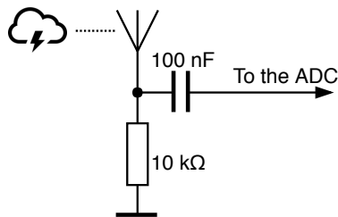
Figure 18.5: The “lightning trap” circuit
