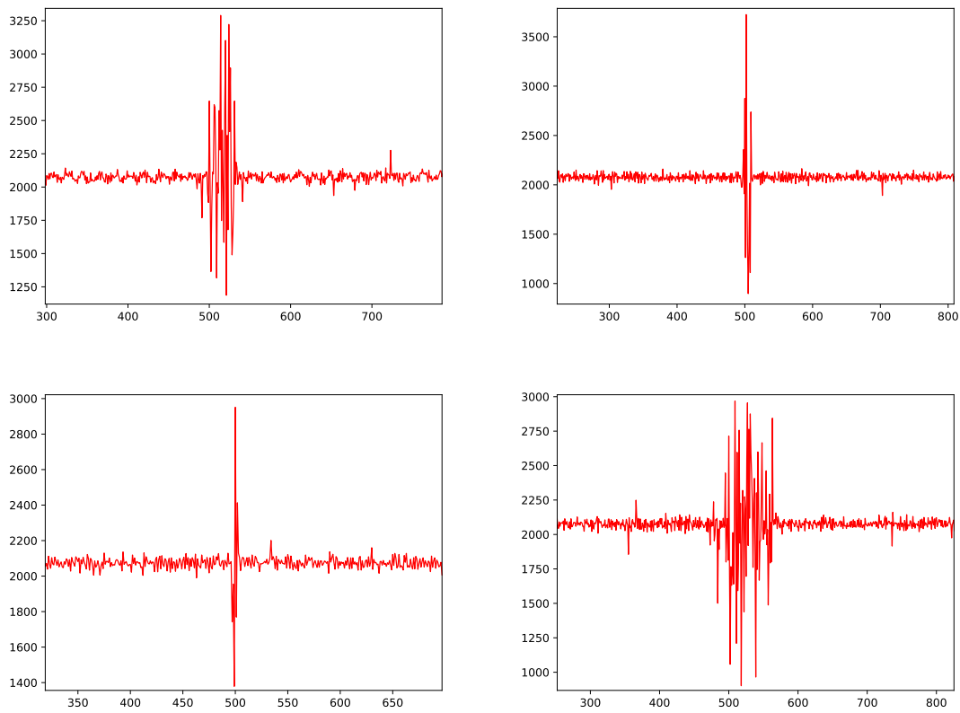
Figure 18.6: Lightning strike-generated bursts of energy captured by the ADC unit. Note the X-axis value 500 where the bursts start: that was the configured pre-trigger length
