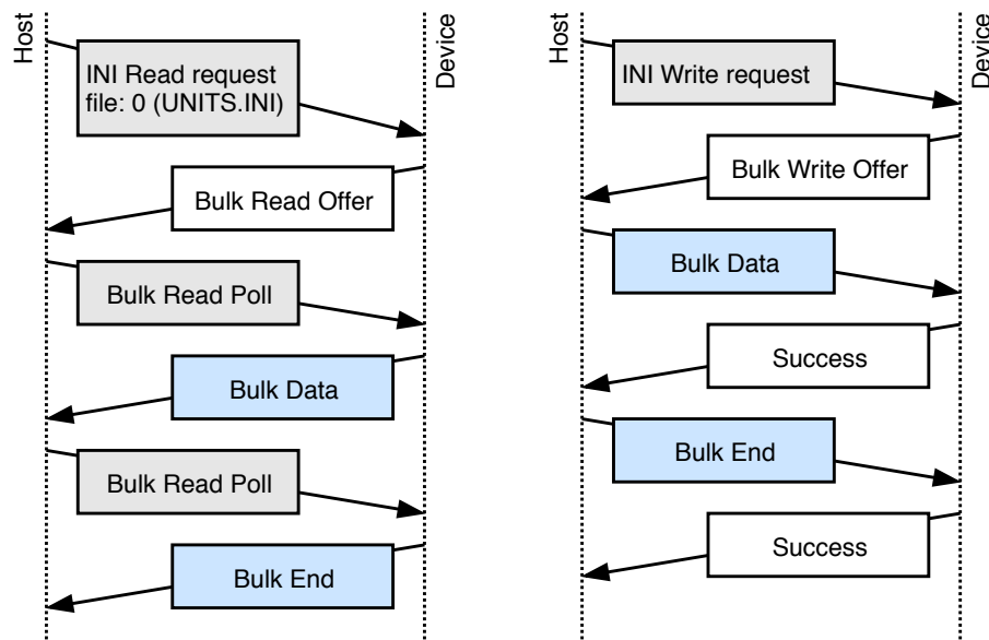
Figure 11.1: A diagram of the bulk read and write transaction.
