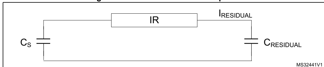
Figure 1. Model of dielectric absorption
