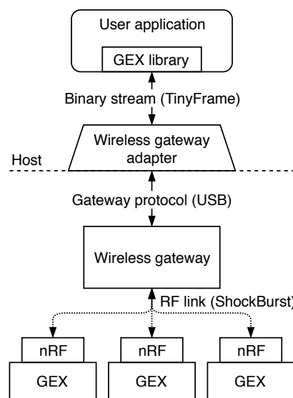
Figure 12.2: A block diagram of the wireless connection
